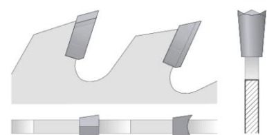
Pointed duplovit tooth
