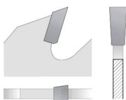
Flat tooth
